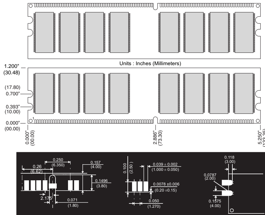
Figure 1: KVR333X64C25K2/1G 184-Pin DIMM
