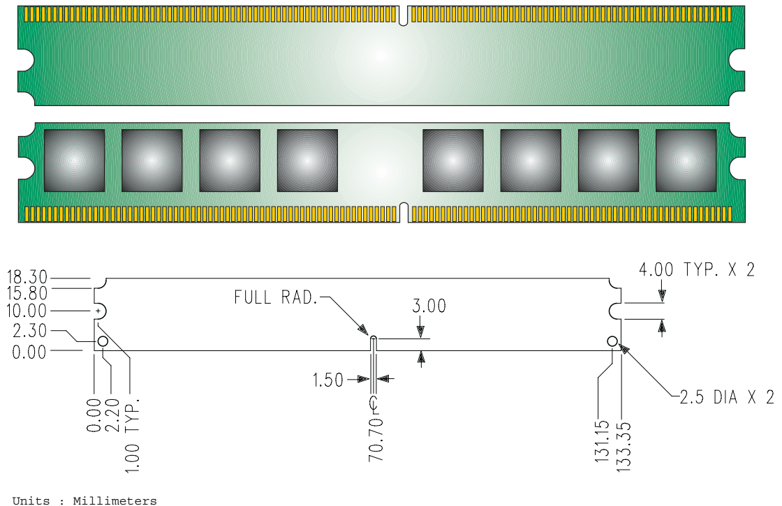
Figure 1: KVR400D2N3K2/2G 240-Pin DIMM
