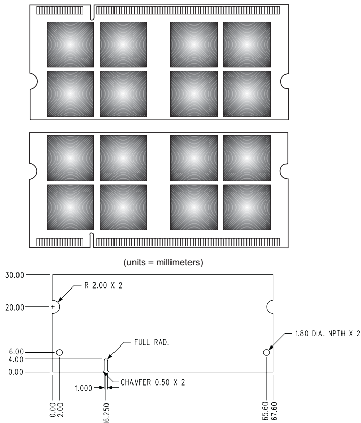
Figure 1: KVR400D2S3/1G 200-Pin SODIMM
