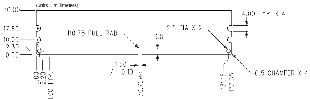
Figure 1: KVR400D2S8R3/1GI 240-Pin DIMM
