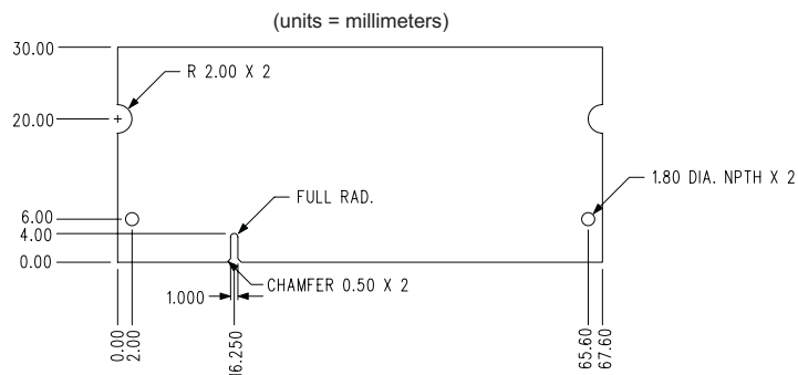
Figure 1: KVR533D2S4/2G 200-Pin SODIMM
