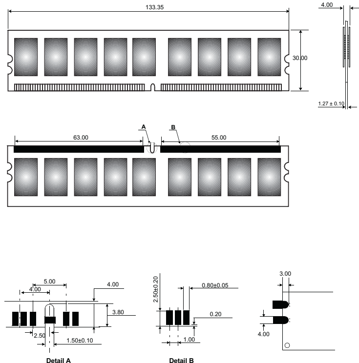
Figure 1: KVR667D2E5K2/4G 240-Pin DIMM
