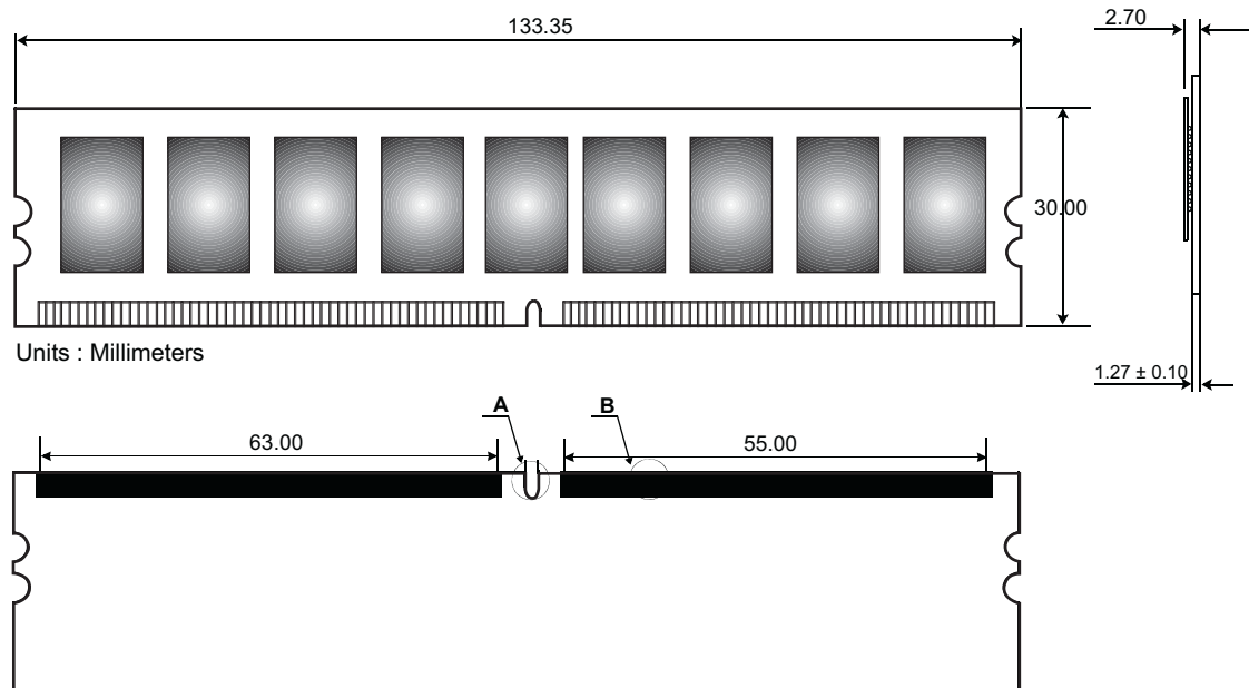
Figure 1: KVR667D2E5/1G 240-Pin DIMM
