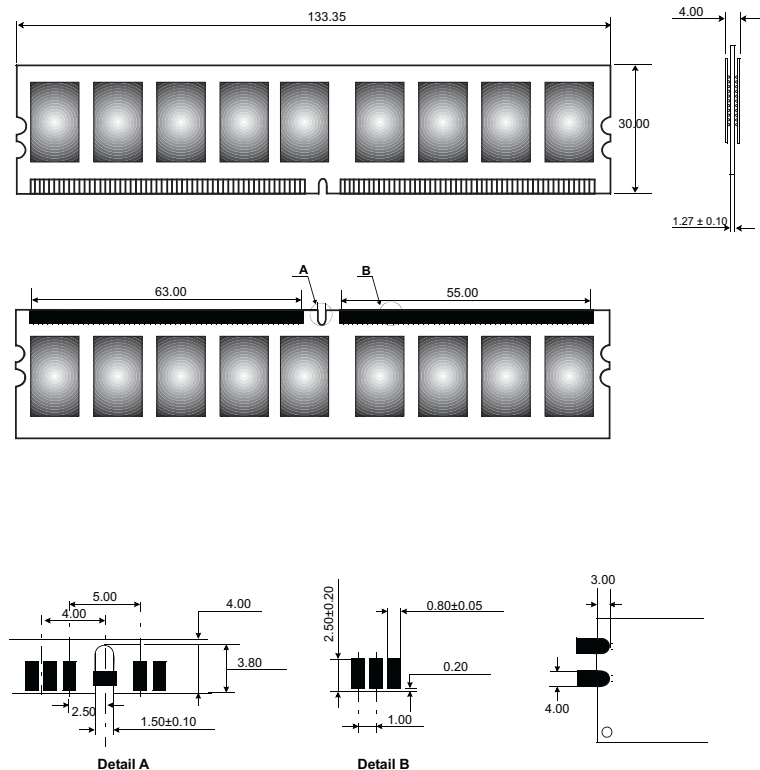
Figure 1: KVR667D2E5/2GI 240-Pin DIMM
