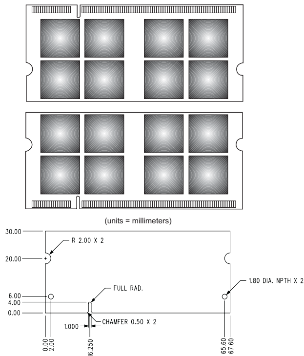
Figure 1: KVR667D2S5K2/2G 200-Pin SODIMM
