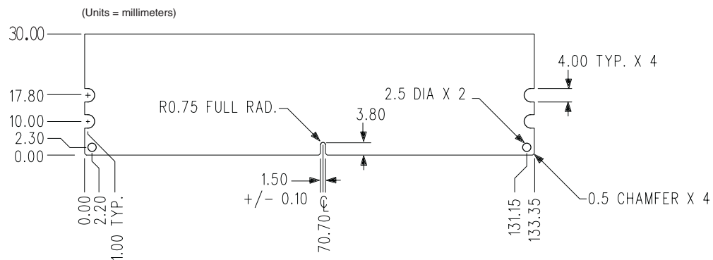
Figure 1: KVR667D2S8P5K2/2G 240-Pin DIMM
