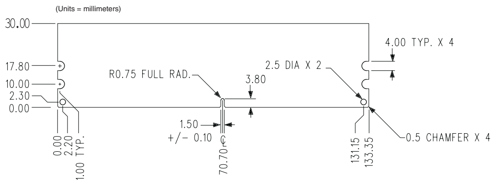
Figure 1: KVR667D2S8P5/1G 240-Pin DIMM
