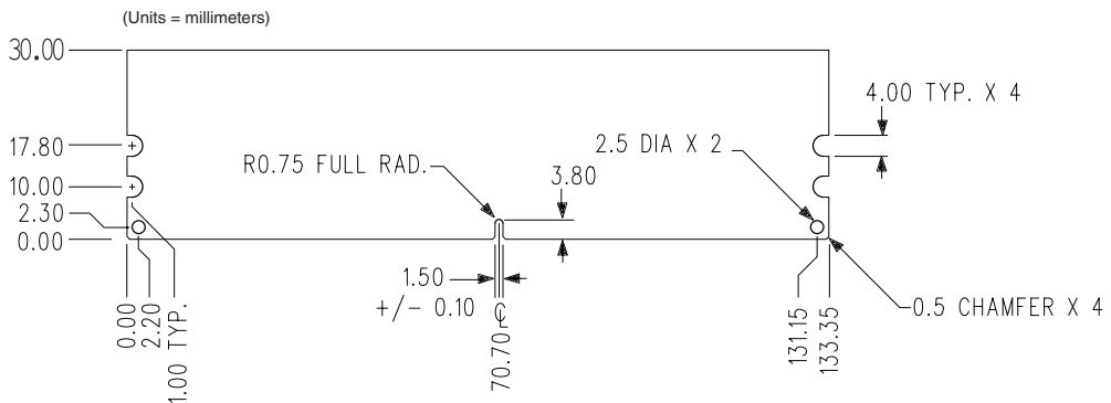
Figure 1: KVR800D2D8P6/2G 240-Pin DIMM
