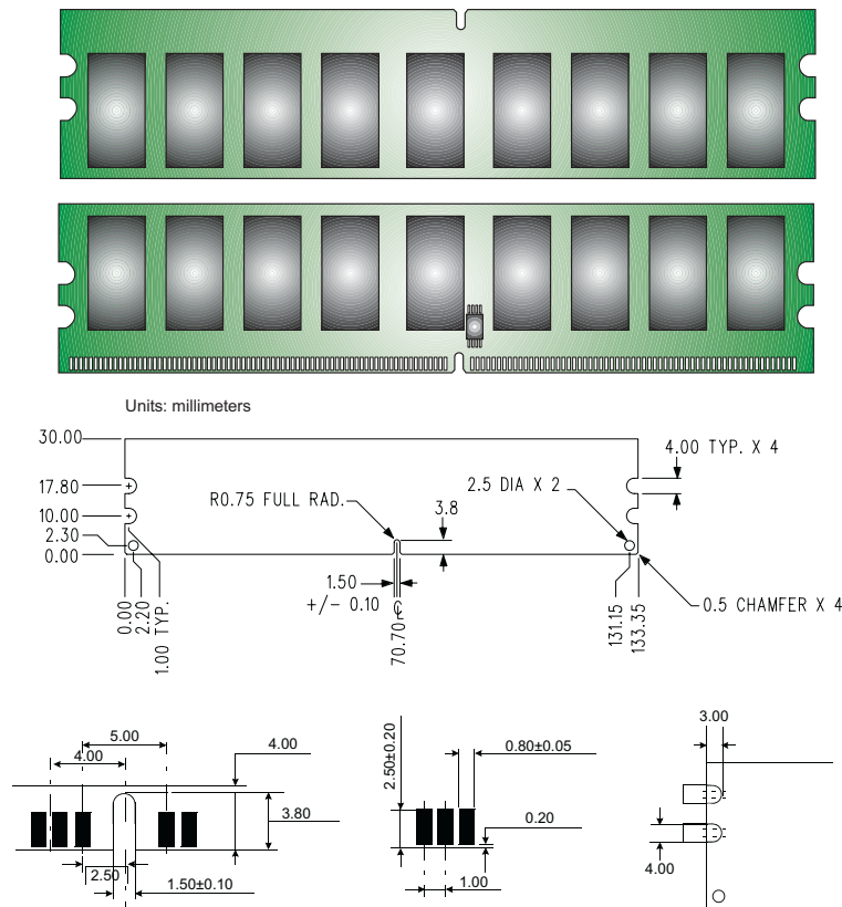
Figure 1: KVR800D2E6/2G 240-Pin DIMM
