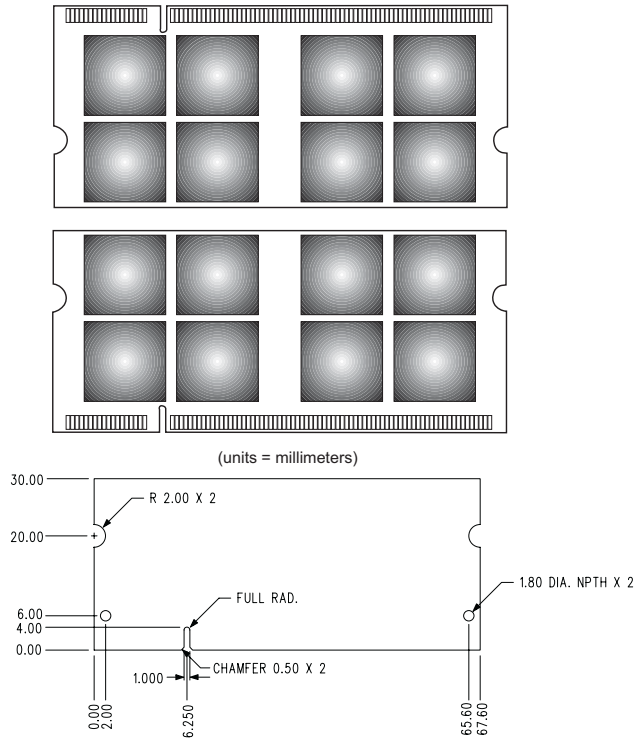
Figure 1: KVR800D2S6/2G 200-Pin SODIMM
